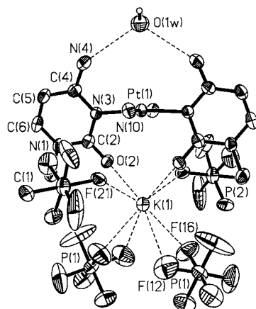
Fig. 2 Section of trans -K[Pt(NH 3 ) 2 (mcyt- N 3 ) 2 ][PF 6 ] 3 ·H 2 O 2 and the atom numbering scheme. Ellipsoids are drawn at the 50% probability level.
