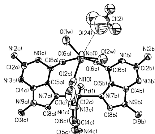
Fig. 3 Section of trans -[Pt(NH 3 )(Hmgua- N 7 ) 2 (mcyt- N 3 )Na(H 2 O) 2 ][ClO 4 ] 3 ·0.5H 2 O 3 with the atom numbering scheme. Ellipsoids are drawn at the 30% probability level.
